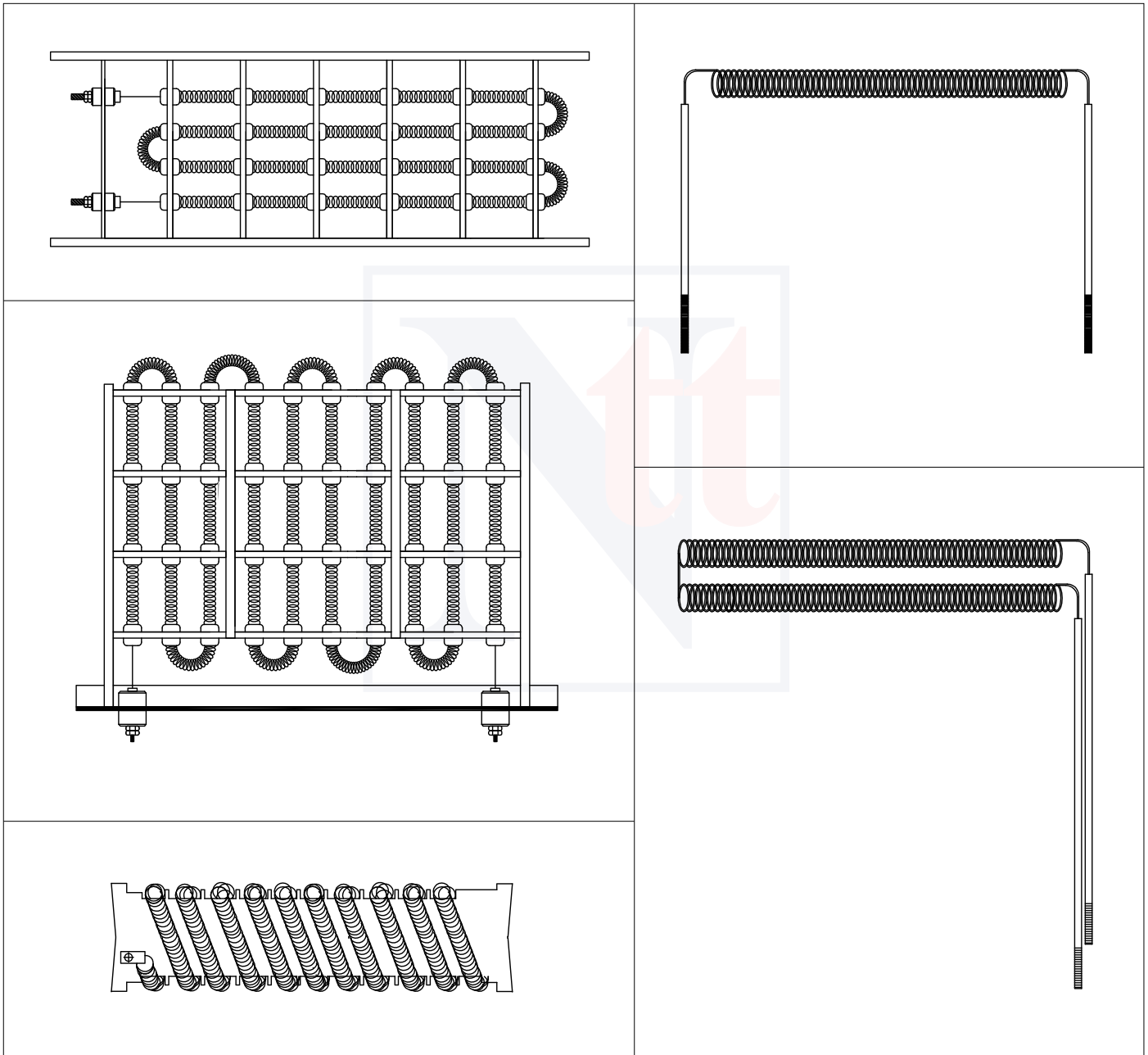
fig. Open Coil Element
